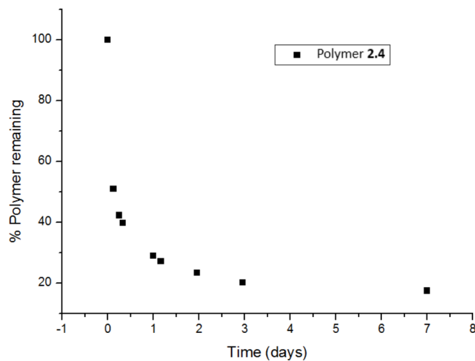
Figure A2. 47 Depolymerization of polymer 2.4 following cleavage of the NVOC end-caps by UV irradiation in 9:1 \text{CD}_3\text{CN}:\text{D}_2\text{O} following by incubation at ambient temperature ( 21^\circ\text{C} ).
