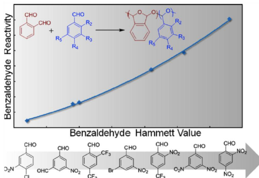
Figure 1. 25 The polymerizability of benzaldehyde derivatives increases with increasing Hammett values. Reproduced with permission from reference 49 .
