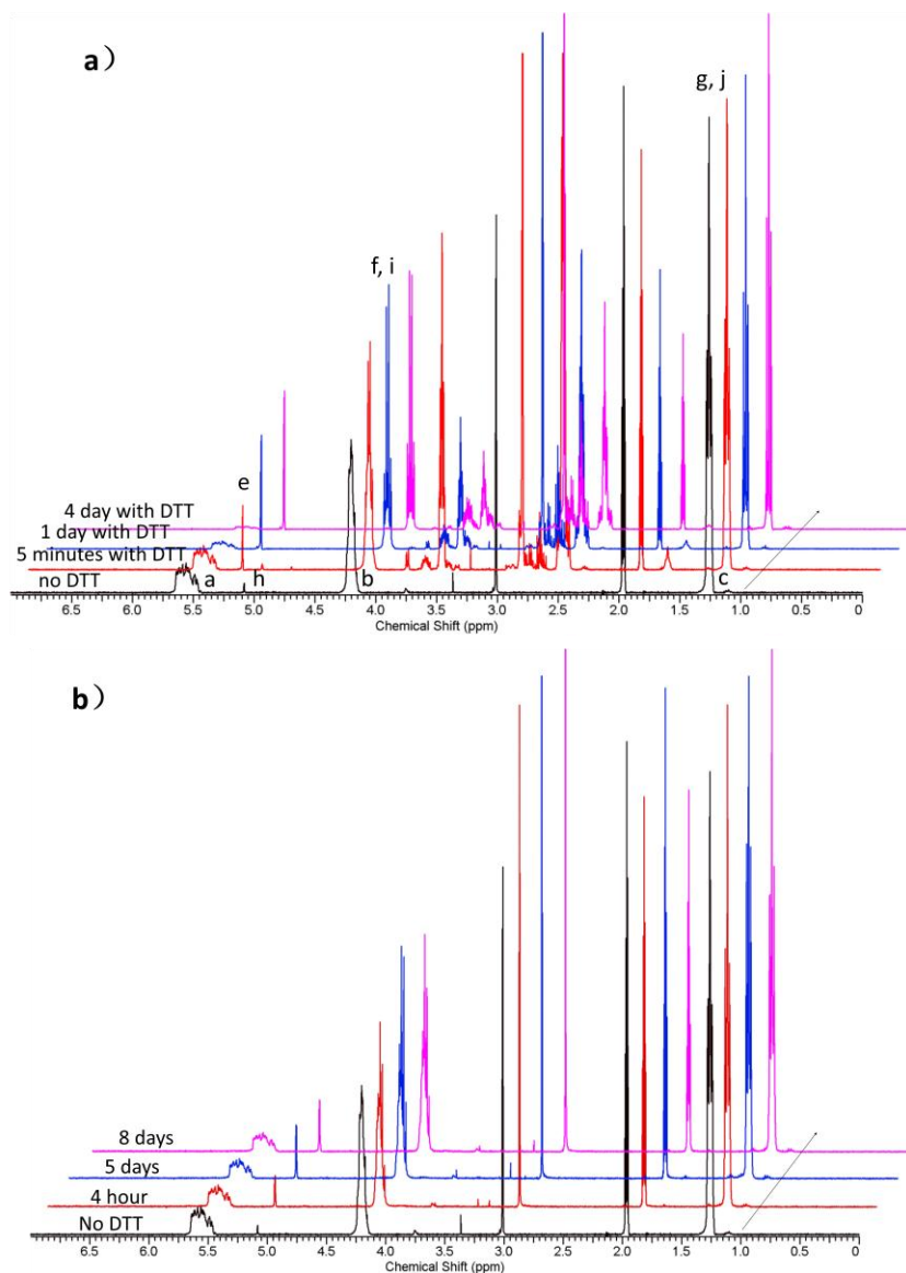
Figure 4.8 1 H NMR spectrum of polymer 4.8 dissolved in 9:1 CD 3 CN:D 2 O with and without addition of DTT. Spectra are offset to allow the progression over time to be clearly observed.
