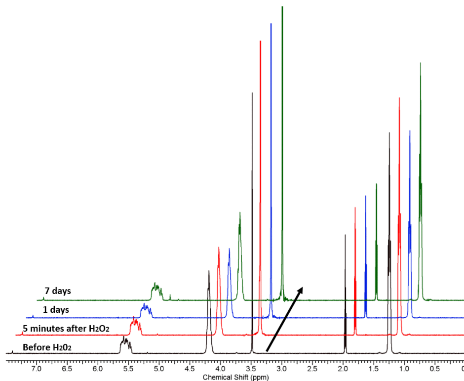
Figure 4. ^3 ^1\text{H} NMR spectra of polymer 2.3 dissolved in 9:1 \text{CD}_3\text{CN}:\text{D}_2\text{O} with addition of \text{H}_2\text{O}_2 . No changes were observed, indicating that the polymer is stable under these conditions and \text{H}_2\text{O}_2 does not cleave the polymer backbone.
