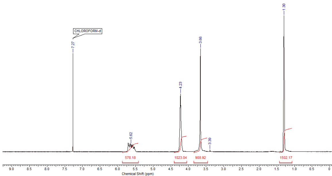
Figure A3. 2 ^1\text{H} NMR spectrum of block polymer (Polymer 3.3) ( \text{CDCl}_3 , 400MHz).
