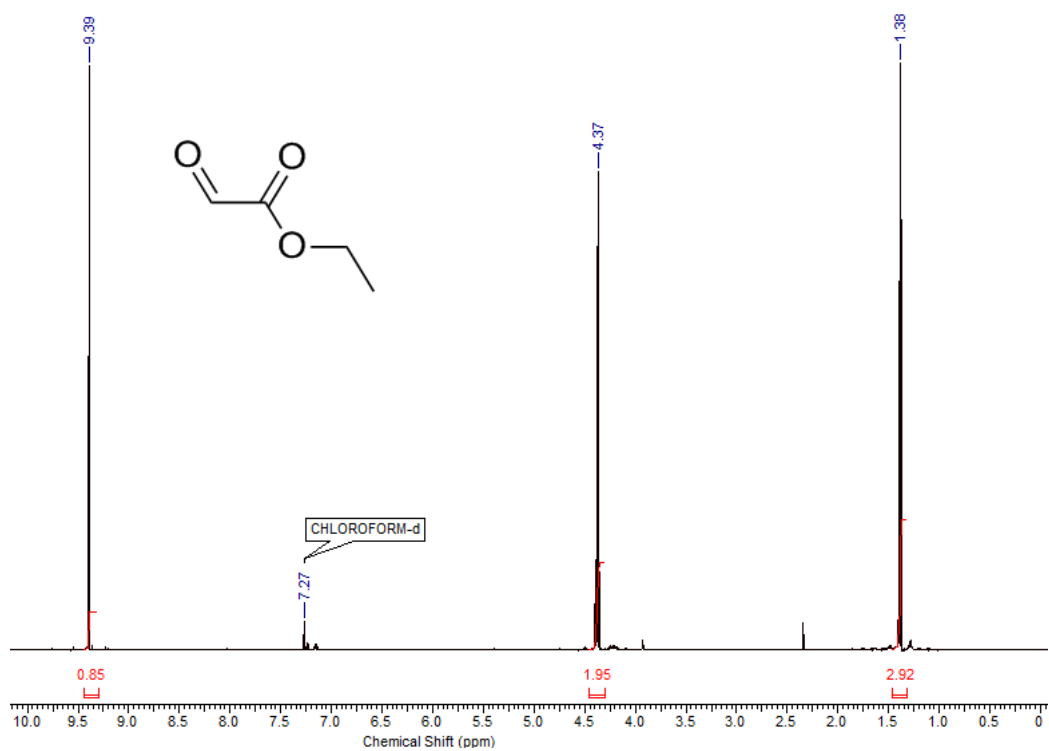
Figure A2. 9 ^1\text{H} NMR spectrum of methyl glyoxylate compound 2.8 ( \text{CDCl}_3 , 400 MHz).
