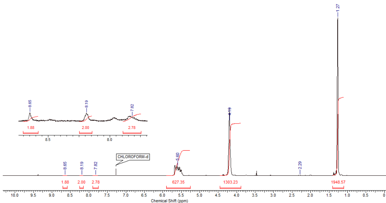
Figure A2. 28 ^1\text{H} NMR spectrum of poly(ethyl glyoxylate) end-capped by compound
