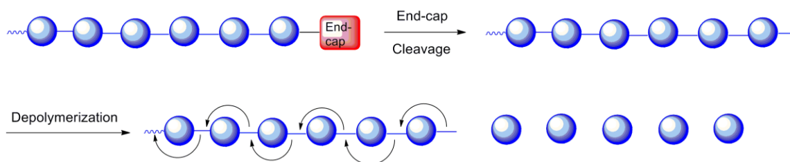
Scheme 4. 1 Degradation mechanism of self-immolative polymer
