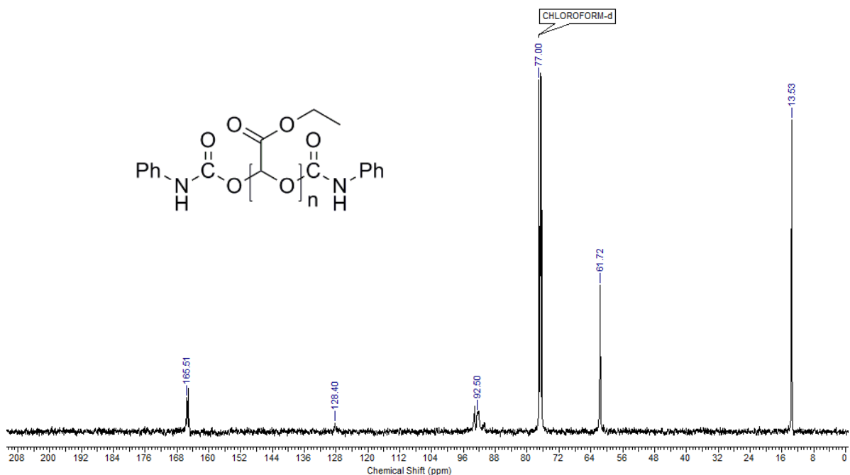
Figure A2. 4 ^{13}\text{C} NMR spectrum of poly(ethyl glyoxylate) end-capped by phenyl isocyanate (Polymer 2.2) ( \text{CDCl}_3 , 150 MHz).
