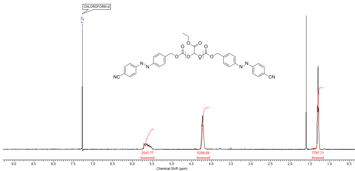
Figure A4. 9 ^1\text{H} NMR spectrum of Polymer 4.9 ( \text{CDCl}_3 , 400 MHz).
