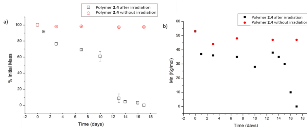
Figure 2.3 a) Mass loss from films of PEtG 2.4 with and without UV irradiation upon incubation in pH 7.4 phosphate buffer. The UV irradiation was conducted in a UV box ( 5 \text{ mW/cm}^3 ) for 17 hours. Error bars represent the standard error of mean on the measurement of 3 films; b) Evolution of molar mass in the same films as measured by SEC (one measurement per time point).
