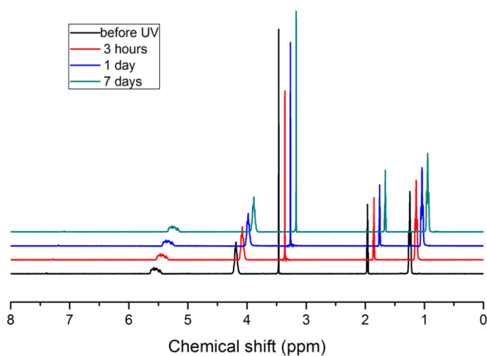
Figure A2. 1 H NMR spectrum of polymer 2.3 after UV irradiation following the same procedure described for the study of polymer 2.4 (following incubation in 9:1 CD 3 CN:D 2 O). No changes were observed, indicating that the polymer is stable under these conditions and UV irradiation does not cleave the polymer backbone.
