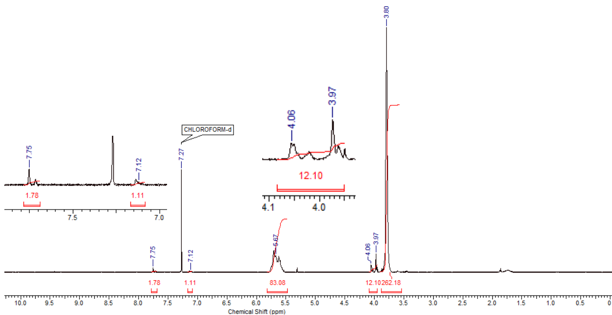
Figure A2. 14 ^1\text{H} NMR spectrum of poly(methyl glyoxylate) end-capped by NVOC-Cl (Polymer 2.11) ( \text{CDCl}_3 , 400 MHz).
