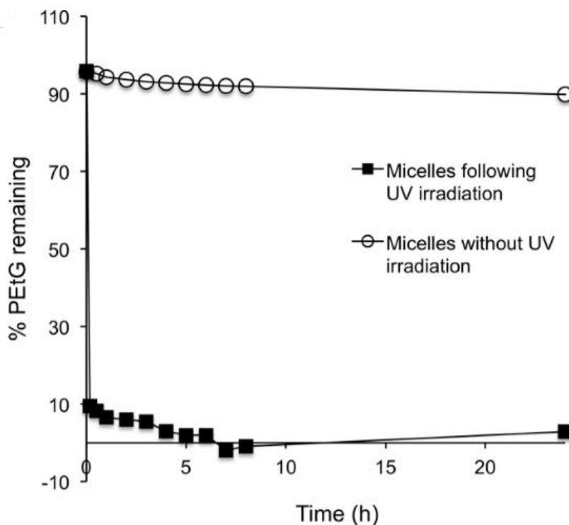
Figure 3. 7 Depolymerization of PEtG in micelles formed from polymer 3.2 following UV irradiation in 5:1 100 mM, pH 7.4 phosphate buffered D_2O:DMSO-d_6 at 37 °C and comparison with a control non-irradiated sample of the micelles
