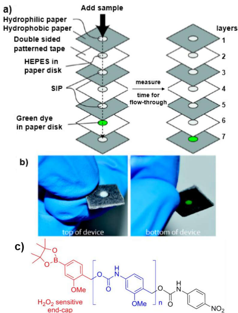
Figure 1. 10 a) Schematic of the design of a phase-switching, time-based assay; b) Observed read-out on the actual device; c) Chemical structure of the SIP employed in this device. Adapted with permission from reference 21 . Copyright 2013 American Chemical Society.
