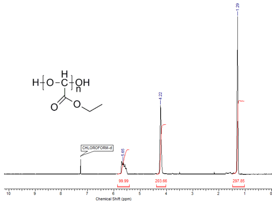
Figure A2. 1 1 H NMR spectrum of poly(ethyl glyoxylate) without end-cap (Polymer 2.1) (CDCl 3 , 400 MHz).
