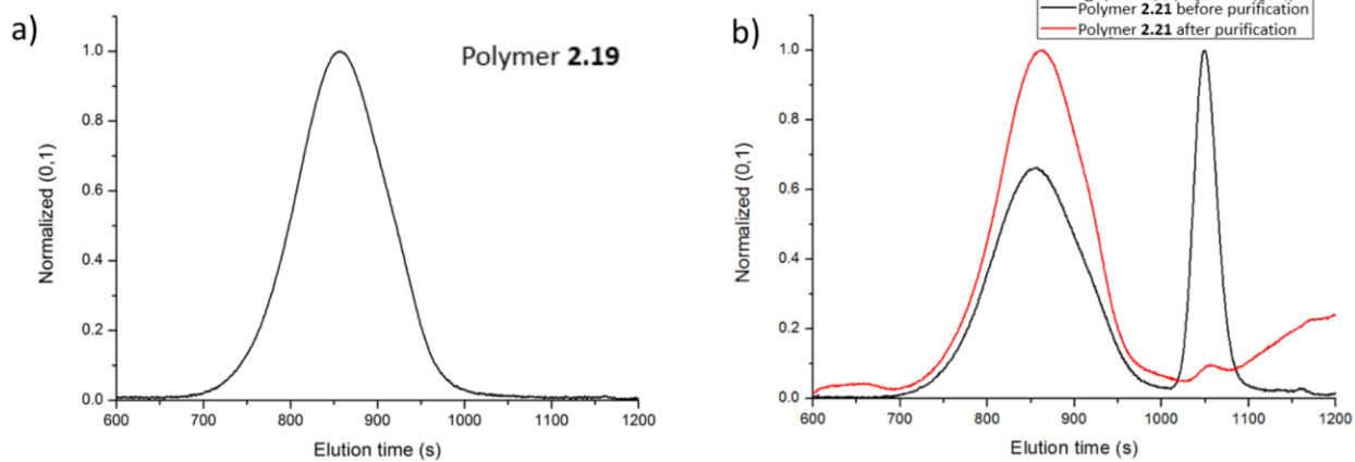
Figure A2. 35 SEC traces for Polymers 2.19 and 2.21
