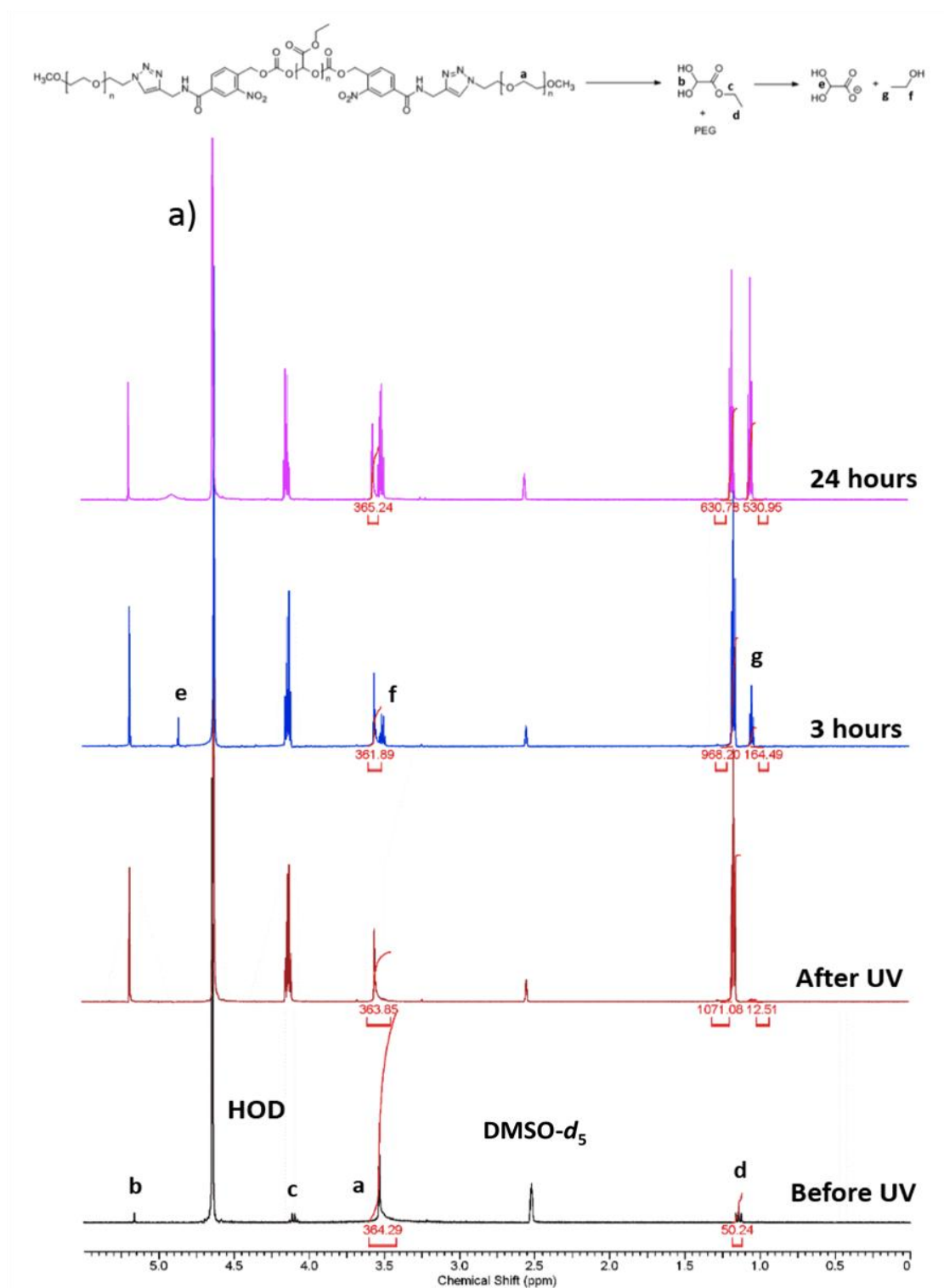
Figure 3. 5 Representative 1 H NMR spectra of micelles over time following UV irradiation and incubation in 5:1 pH 7.4 phosphate buffered D 2 O:DMSO- d 6 .
