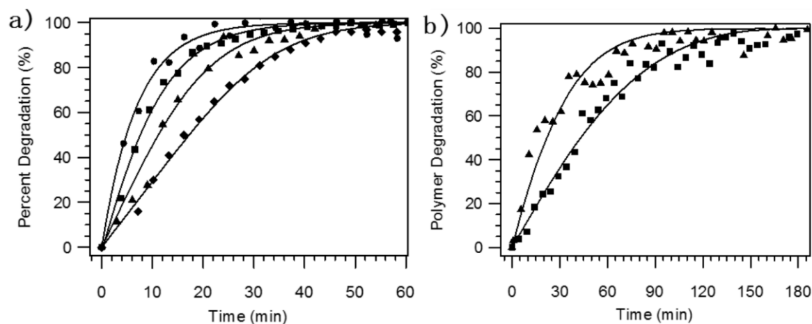
Figure 1.30 Degradation kinetics of as measured by ^1\text{H} NMR spectroscopy in 0.1 M phosphate buffer ( \text{D}_2\text{O} ):acetone- d_6 (3:2) at 37^\circ\text{C} . a) Monomer ( \bullet ), dimer ( \blacksquare ), tetramer ( \blacktriangle ), octamer ( \blacklozenge ). Solid lines correspond to the regressed fits of Eq. (7). b) Degradation kinetics of polymers M_n = 5250 g/mol with D of 1.47 ( \blacktriangle ) and M_n = 13,600 g/mol with D of 1.58 ( \blacksquare ). Overlaid lines correspond to the self-immolative model fits for both polymers. Reproduced with permission from reference 67 .
