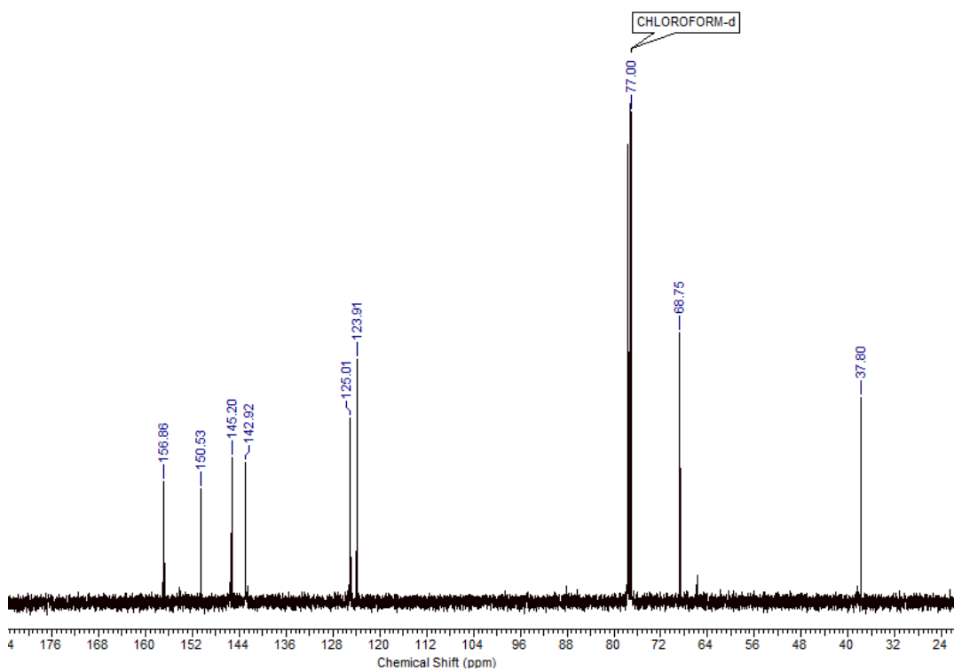
Figure A4. 3 ^{13}\text{C} NMR spectrum of Chloroformate 4.5 ( \text{CDCl}_3 , 150 MHz).
