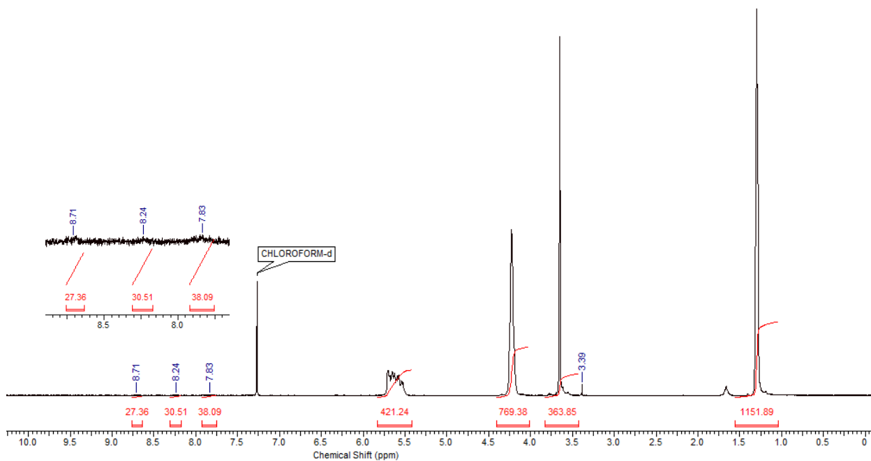
Figure A2. 30 ^1\text{H} NMR spectrum of block polymer (Polymer 2.21) ( \text{CDCl}_3 , 400MHz).
