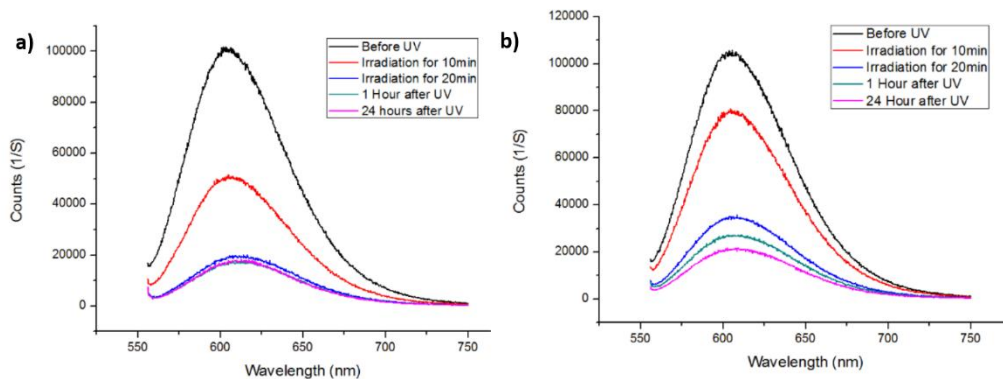
Figure 3.10 Changes in fluorescence intensity of Nile red with different irradiation times of micelles at a) pH 7.4 and b) pH 5.0, the sample was incubated at 37 °C.
