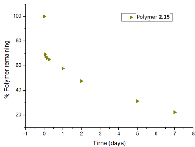
Figure A2. 52 Depolymerization of polymer 2.15 following cleavage of the NVOC end-caps by UV irradiation in 9:1 CD 3 CN:D 2 O following incubation at ambient temperature (21°C).
