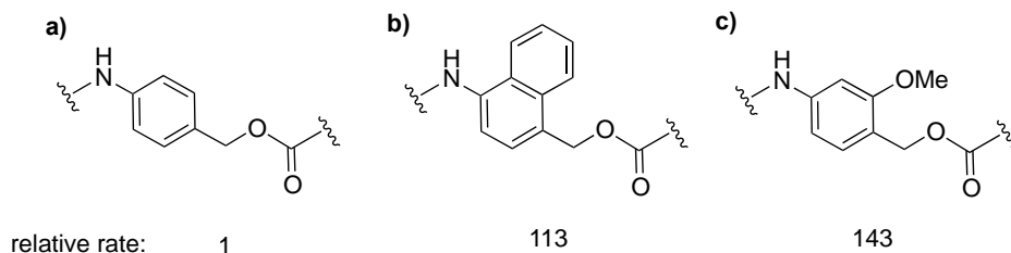
Figure 1. 11 Chemical structures of 4-aminobenzyl alcohol derivatives with increased rates of 1,6-elimination: a) parent structure; b) naphthalene derivative; c) methoxy derivative.
