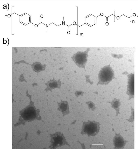
Figure 1. 16 a) Chemical structure of an amphiphilic self-immolative block copolymer; b) Transmission electron microscopy image of assemblies of this block copolymer formed in aqueous solution (scale bar = 100 nm). Adapted with permission from reference 32 . Copyright 2009 American Chemical Society.
