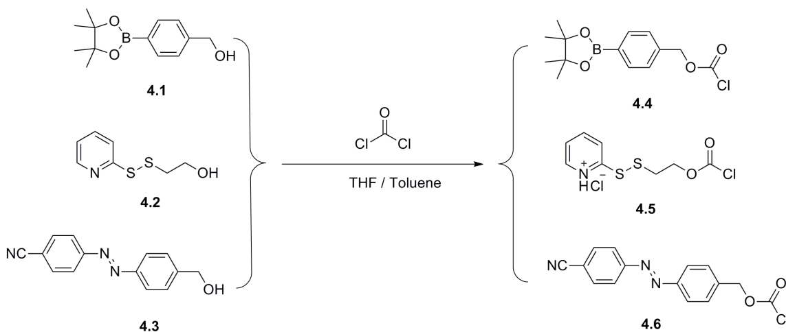
Scheme 4. 2 Synthesis of chloroformate based end-caps.
